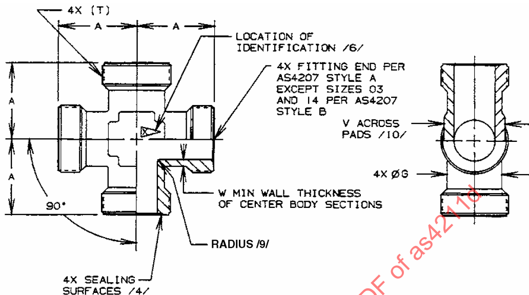
FIGURE 1 - FITTING, CROSS
