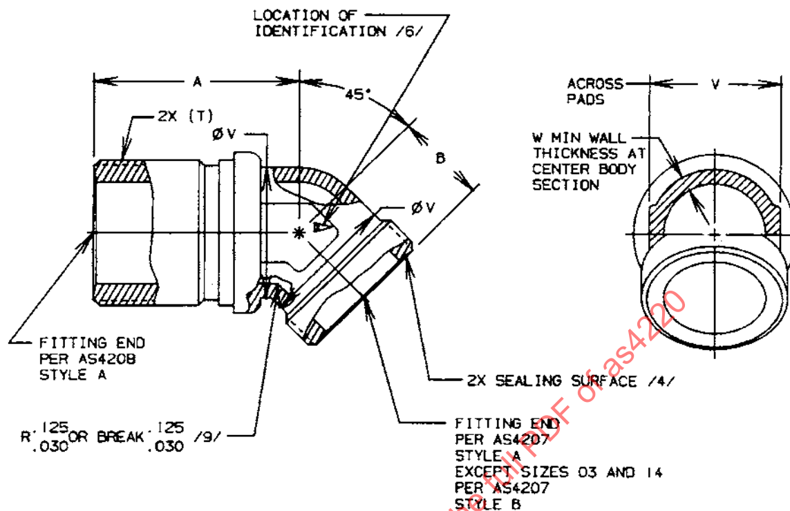
FIGURE 1 - FITTING, ELBOW, 45°, BULKHEAD
