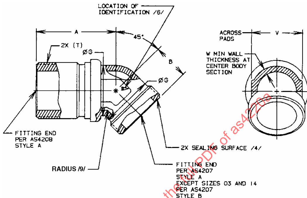
FIGURE 1 - FITTING, ELBOW, 45°, BULKHEAD
