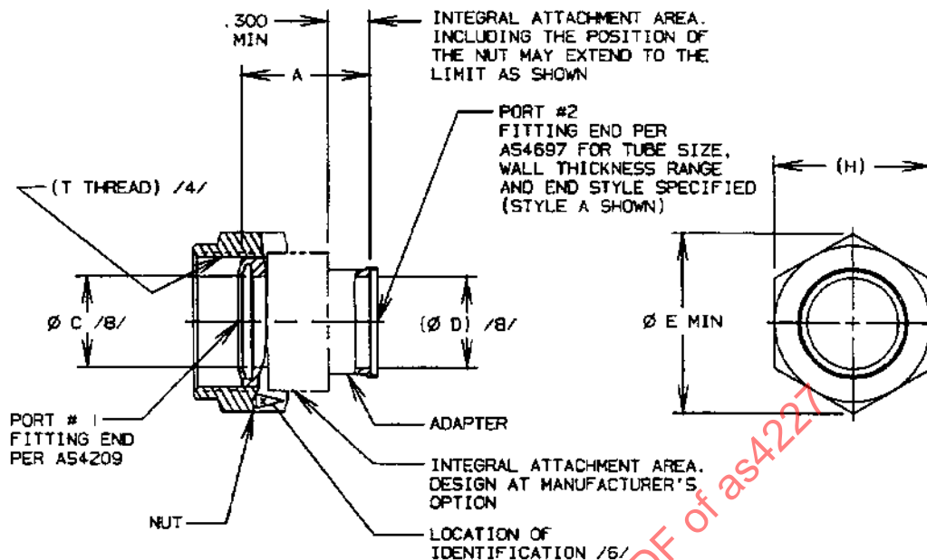
FIGURE 1 - FITTING ASSEMBLY, ADAPTER
