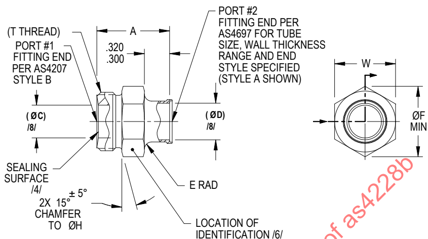
FIGURE 1 - FITTING, ADAPTER
