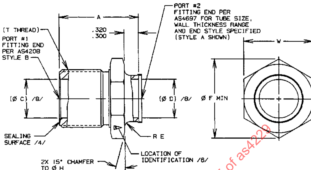
FIGURE 1 - FITTING, ADAPTER, BULKHEAD
