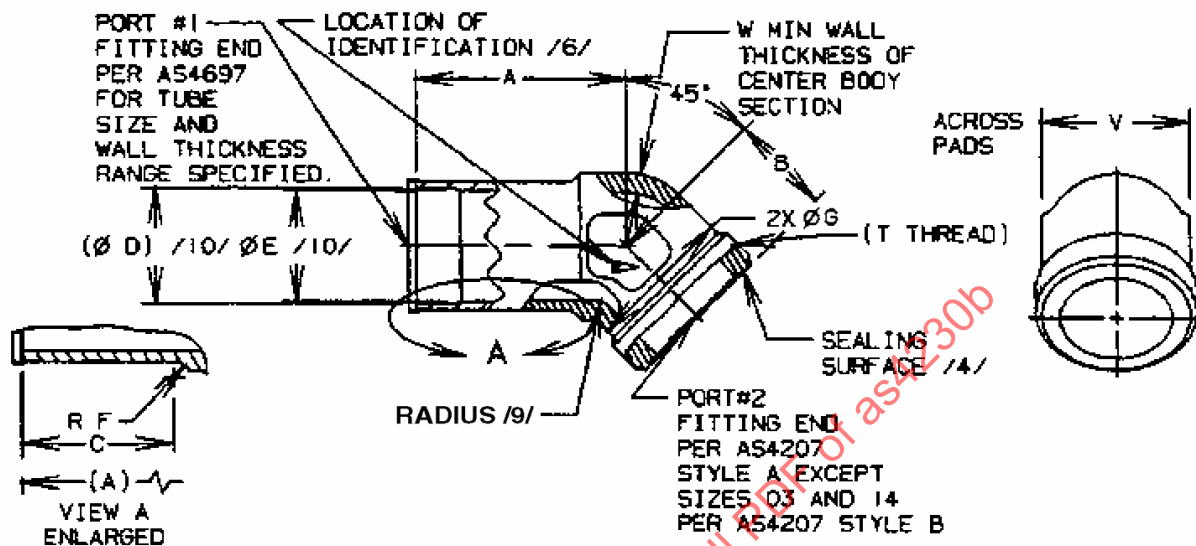
FIGURE 1 - FITTING, ELBOW, 45°
