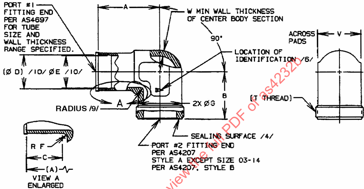
FIGURE 1 - FITTING, ELBOW, 90°
