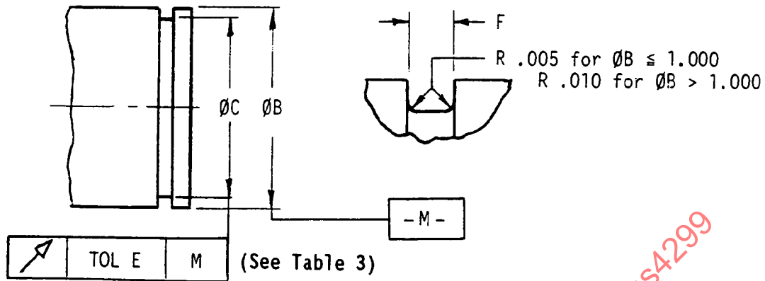
FIGURE 2 - Groove Dimensions, Type I, Classes 1 and 2 Retaining Rings (See Table 4)
