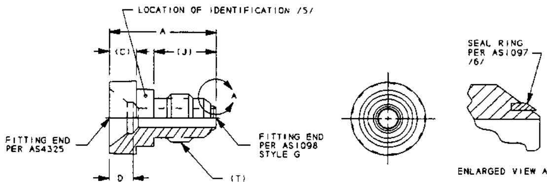
FIGURE 1 - REDUCER, ADAPTER, CONICAL END TO FLARED TUBE
