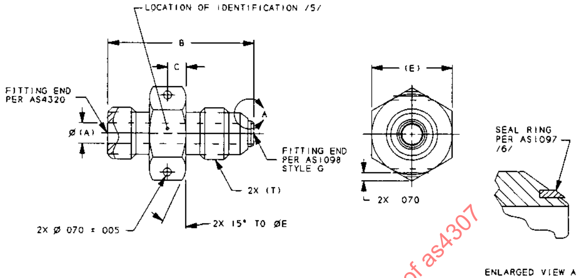
FIGURE 1 - ADAPTER, FLARED TUBE TO BOSS
