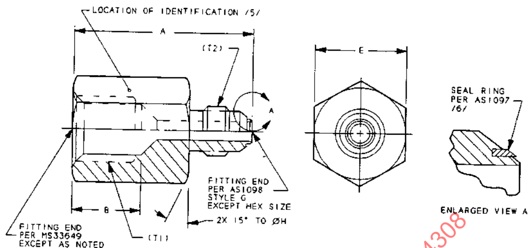
FIGURE 1 - BUSHING, SCREW THREAD EXPANDER
