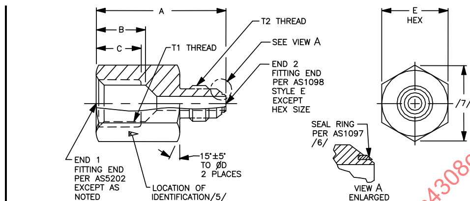
FIGURE 1 - FITTING, BUSHING-SCREW THREAD EXPANDER
