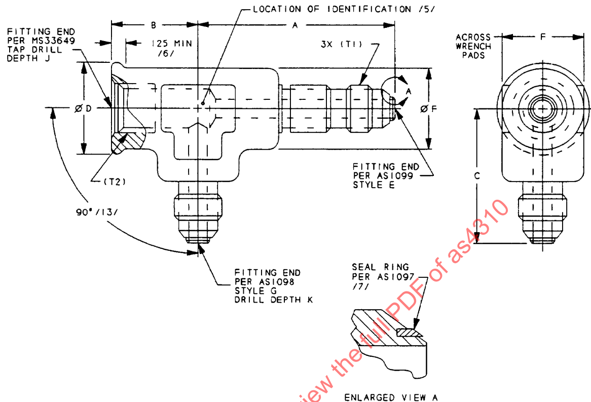
FIGURE 1 - TEE, FLARED TUBE, INTERNAL THREAD ON RUN
