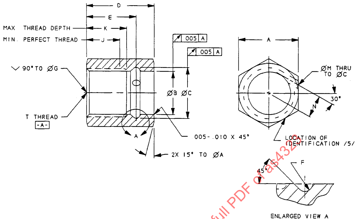
FIGURE 1 - SWIVEL NUT
