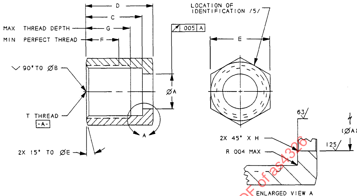
FIGURE 1 - NUT, COUPLING
