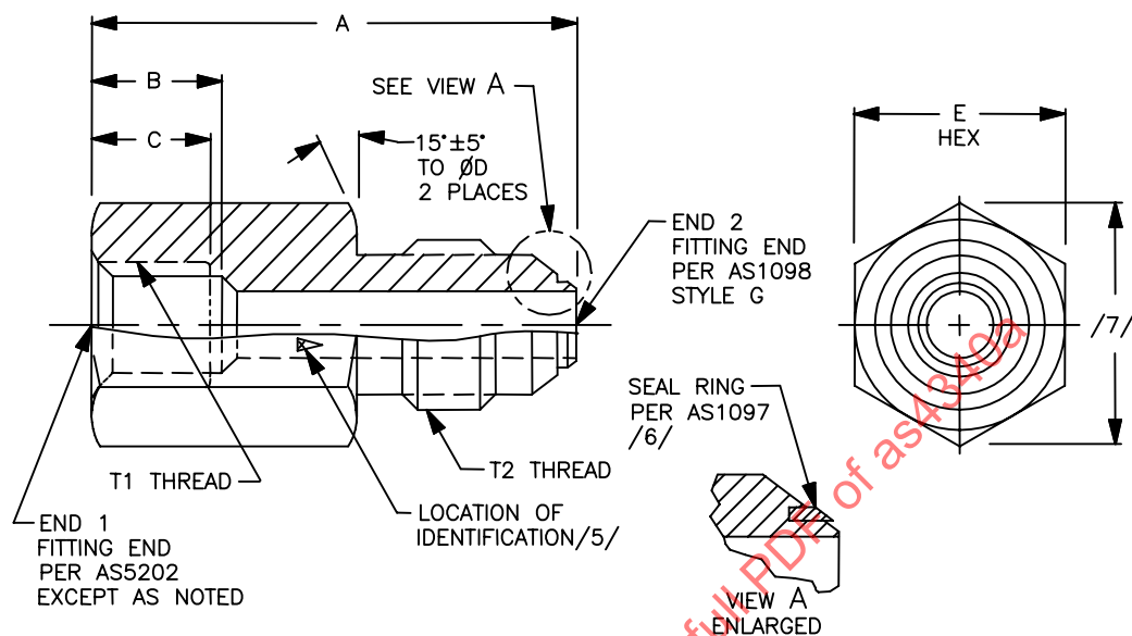
FIGURE 1 - FITTING, BUSHING, SCREW THREAD REDUCER
