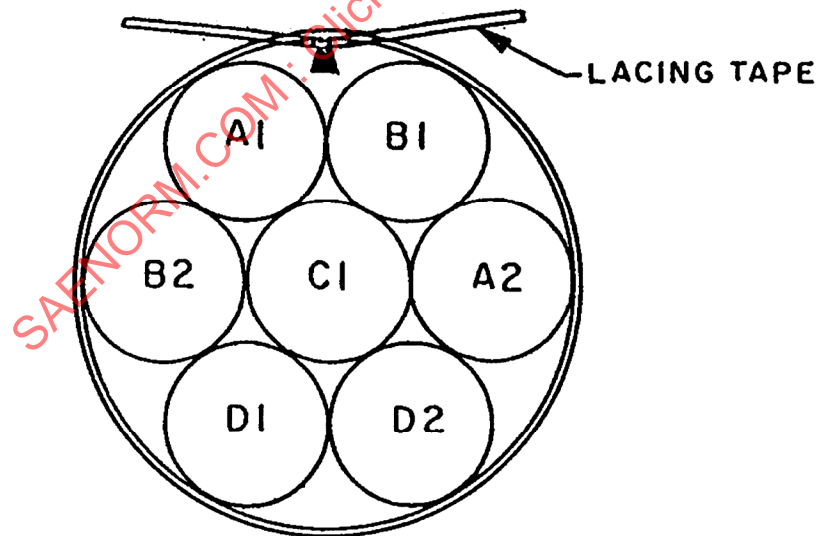
FIGURE 8 - BUNDLE CONFIGURATION
