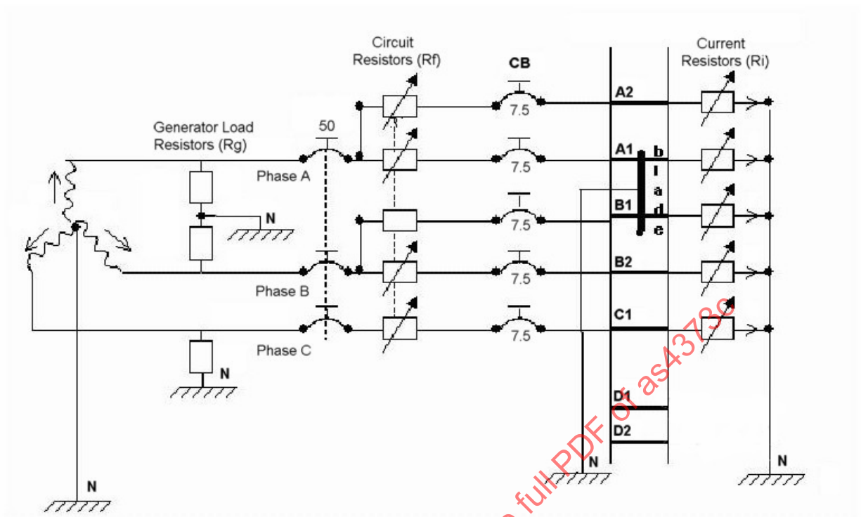
FIGURE 11 - ELECTRICAL CONNECTION
