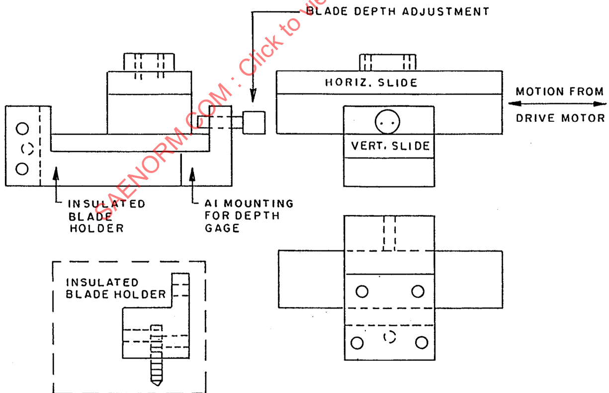
FIGURE 12 - BALL SLIDE BLADE FIXTURE
