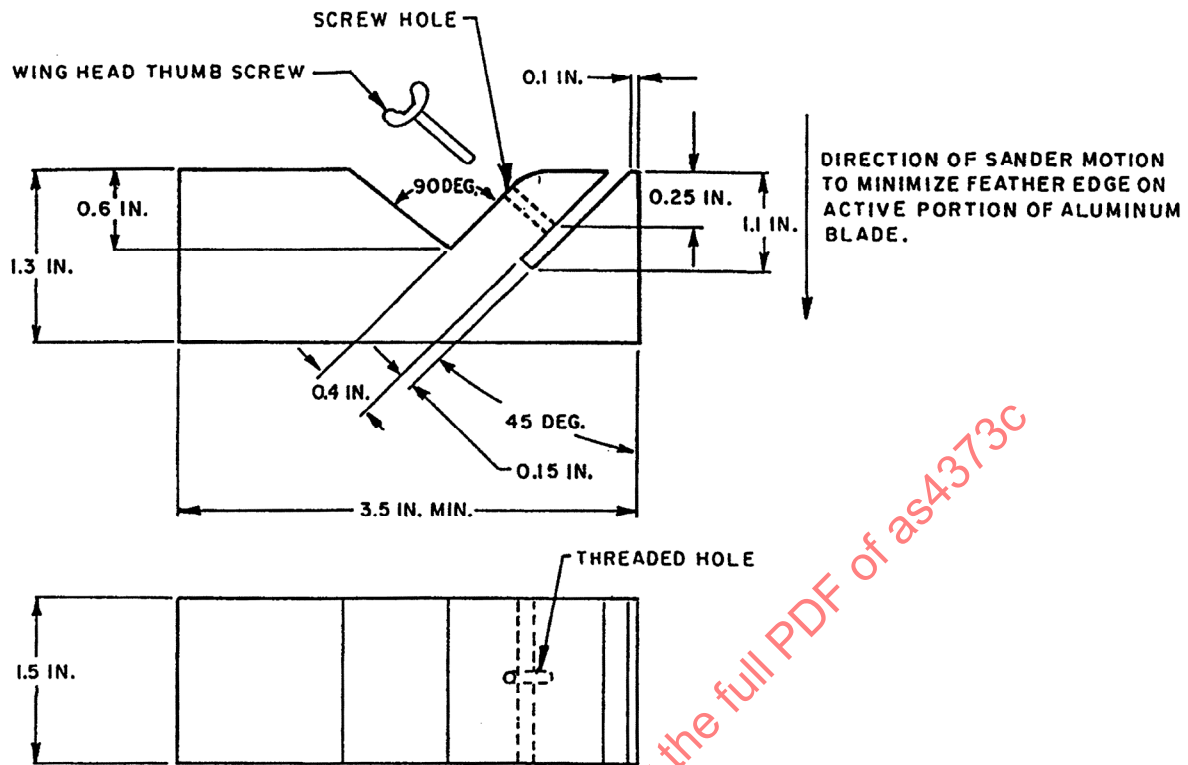
FIGURE 7 - ALUMINUM BLADE SHARPENING FIXTURE
