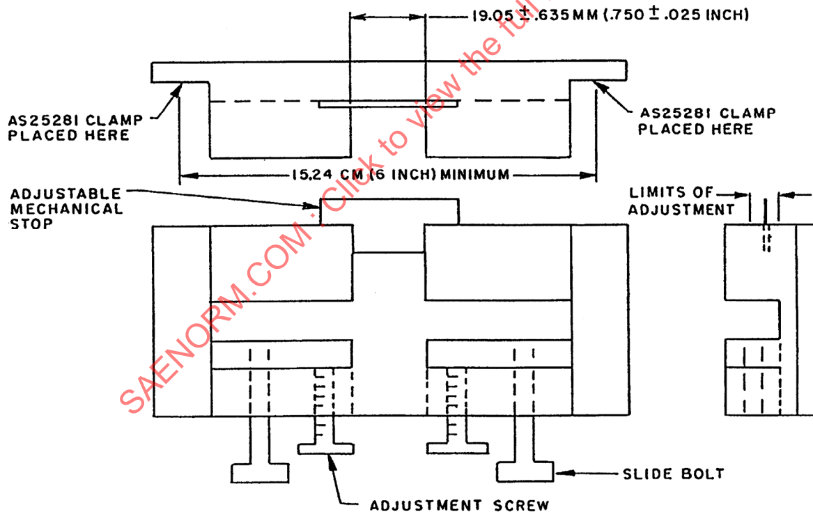
FIGURE 10 - TEST FIXTURE
