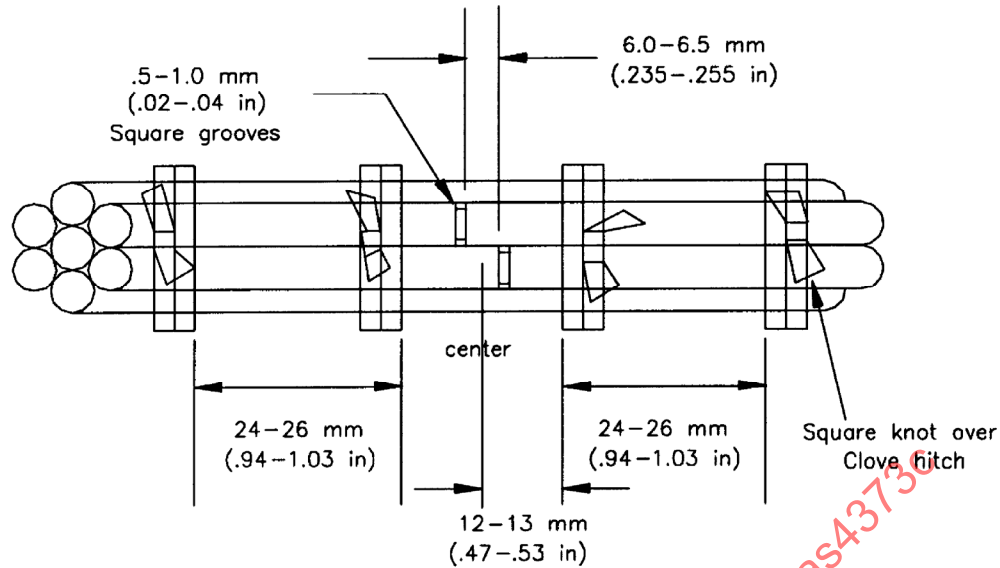
FIGURE 14 - BUNDLE TYING
