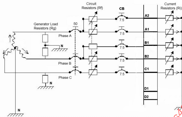
FIGURE 15 - ELECTRICAL CONNECTION
