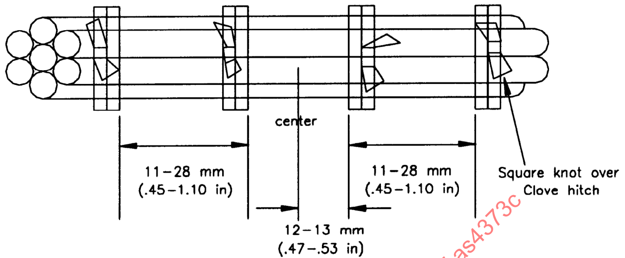
FIGURE 9 - BUNDLE TYING
