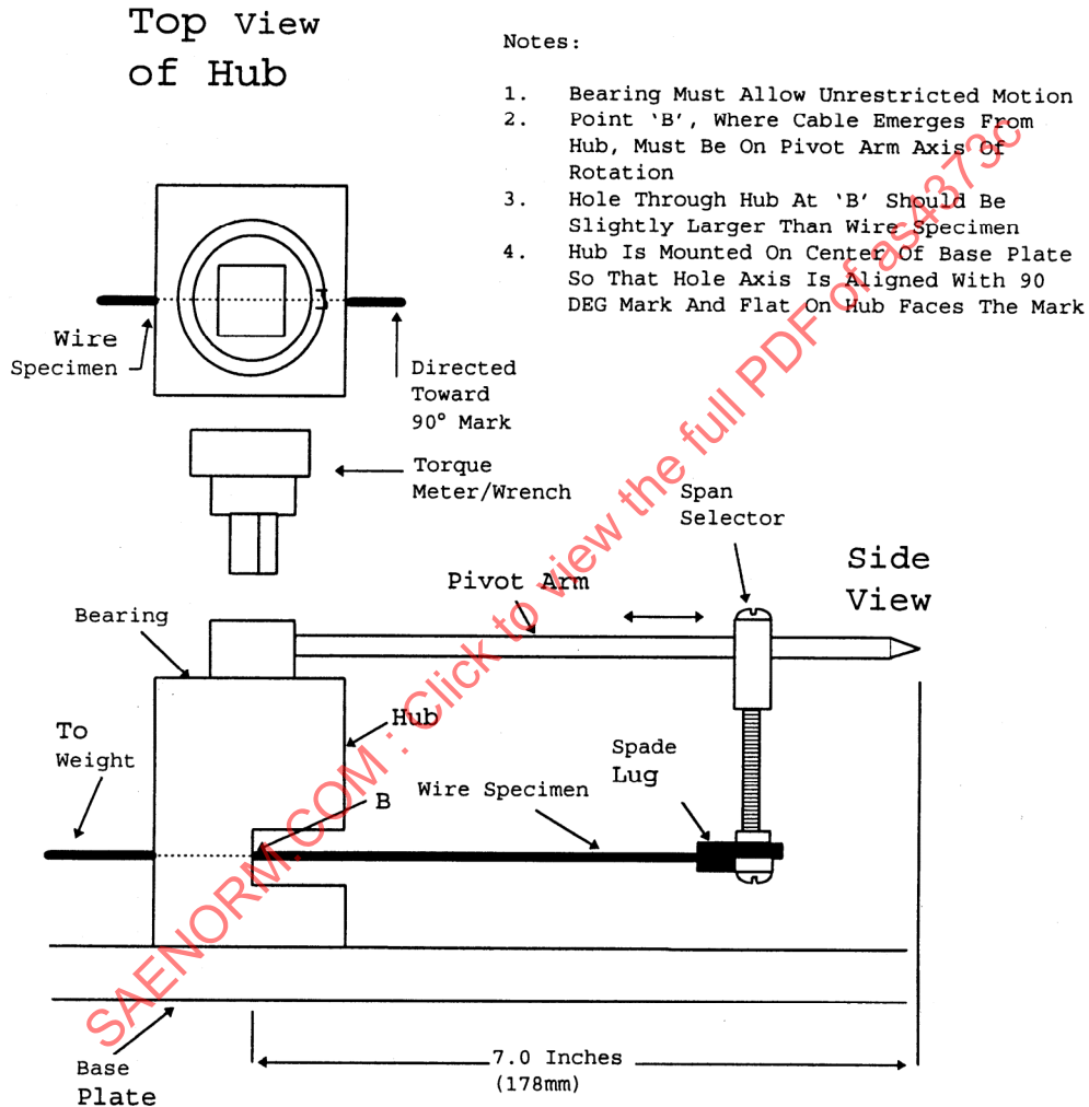
FIGURE 18 - TEST FIXTURE FOR STIFFNESS AND SPRINGBACK TEST
