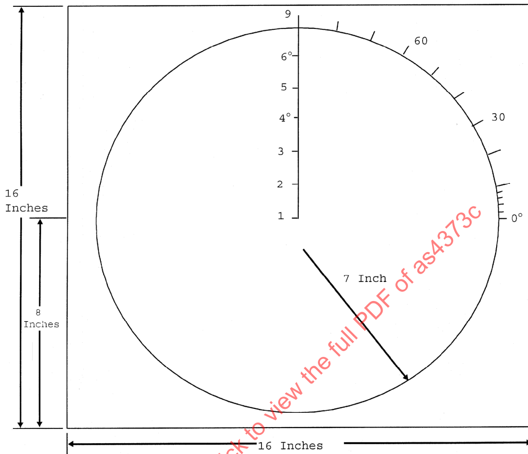
FIGURE 19 - STIFFNESS AND SPRINGBACK TEST FIXTURE BASE PLATE
