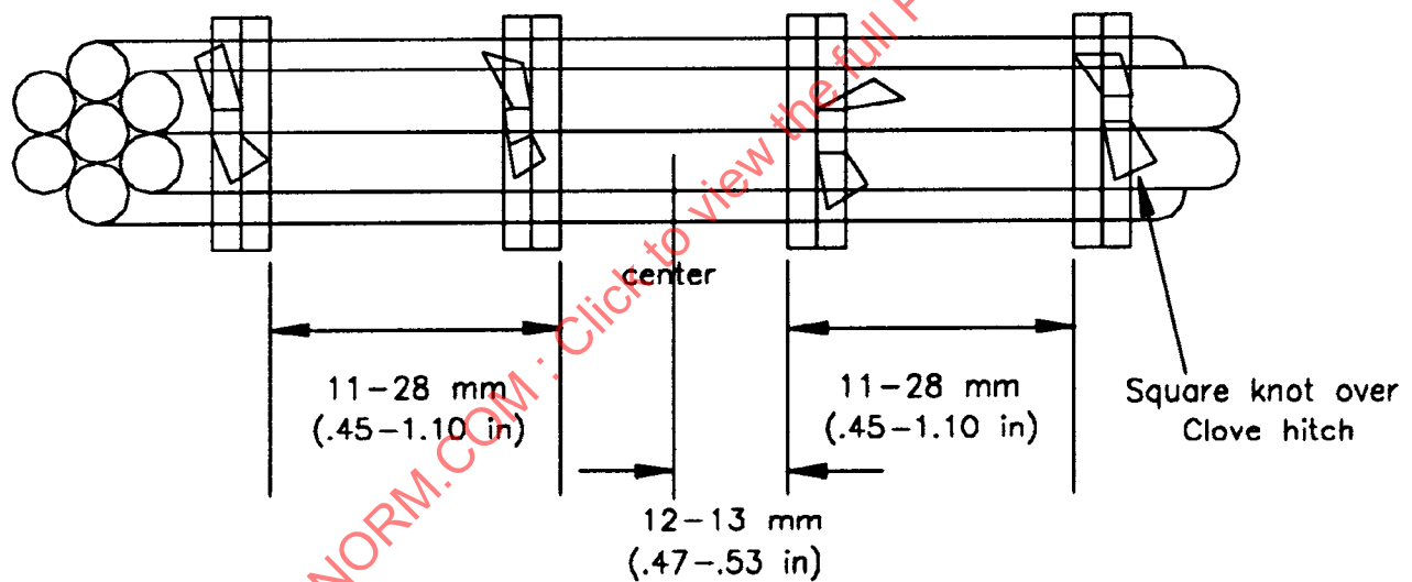
FIGURE11 - BUNDLE TYING
