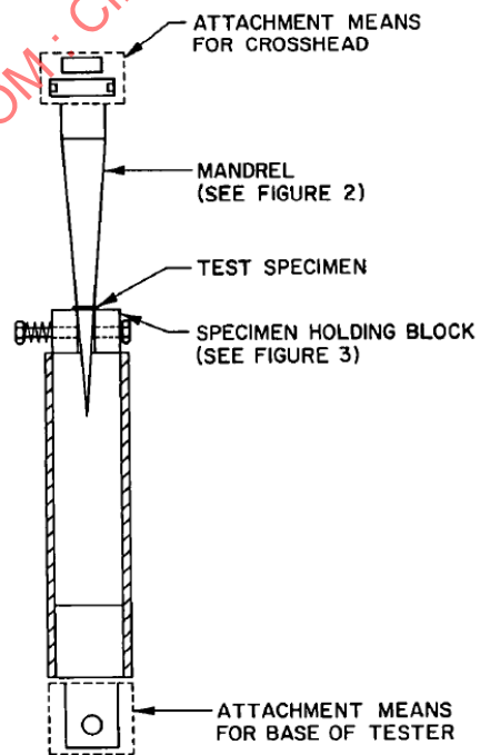
FIGURE 25 – CIRCUMFERENTIAL ELONGATION APPARATUS
