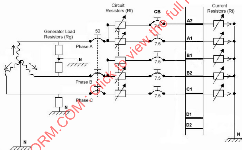
FIGURE 17 - ELECTRICAL CONNECTION
