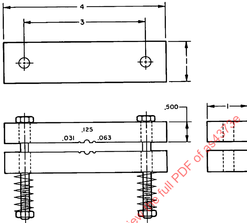
FIGURE 27 – SPECIMEN HOLDING BLOCK
