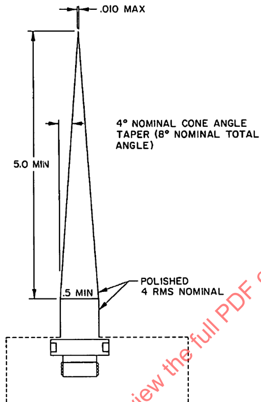
FIGURE 25 – CIRCUMFERENTIAL ELONGATION APPARATUS
