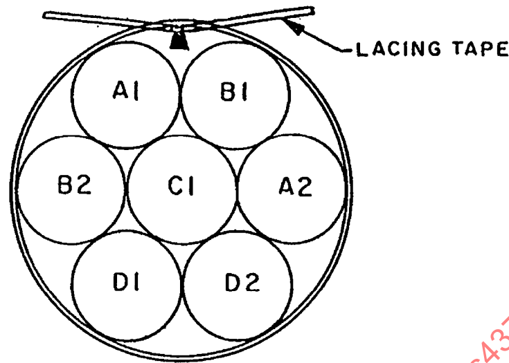
FIGURE 15 - BUNDLE CONFIGURATION
