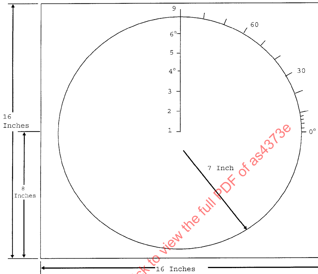
FIGURE 22 - STIFFNESS AND SPRINGBACK TEST FIXTURE BASE PLATE
