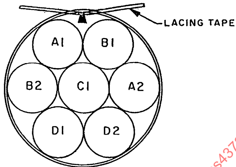
FIGURE10 - BUNDLE CONFIGURATION
