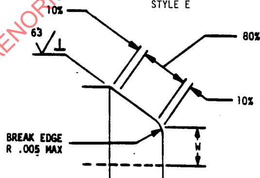
FIGURE 3 - ENLARGED VIEW A
