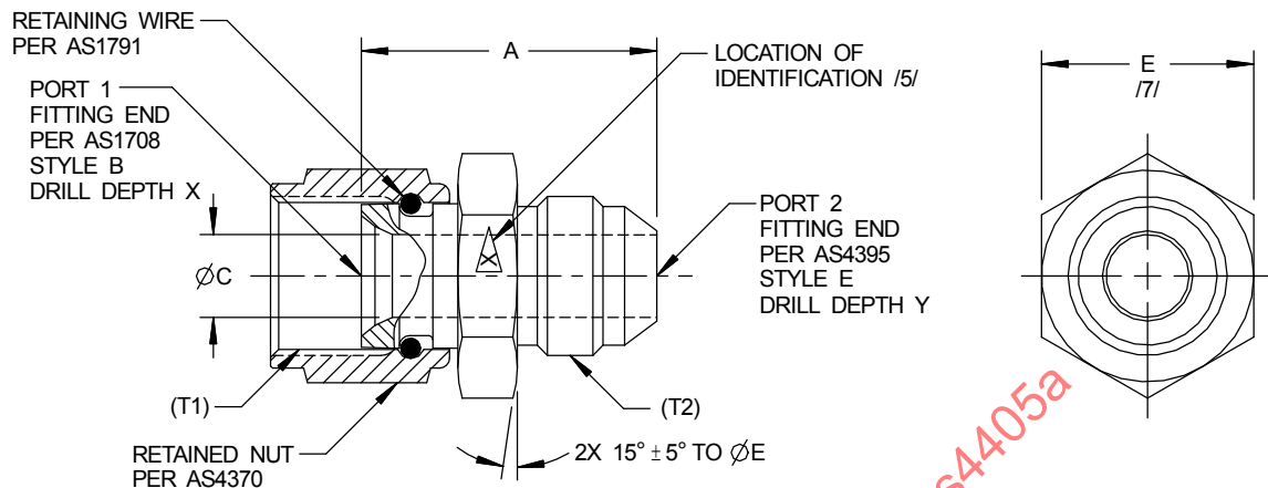
FIGURE 1 - FITTING ASSEMBLY, ADAPTER
