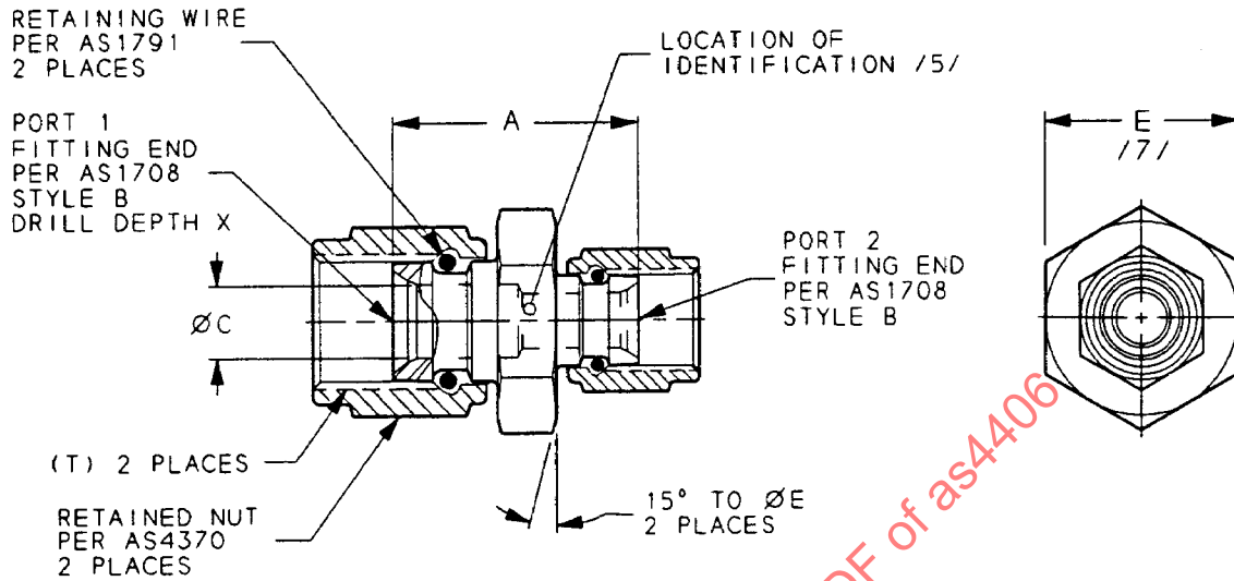
FIGURE 1 - FITTING ASSEMBLY, UNION
