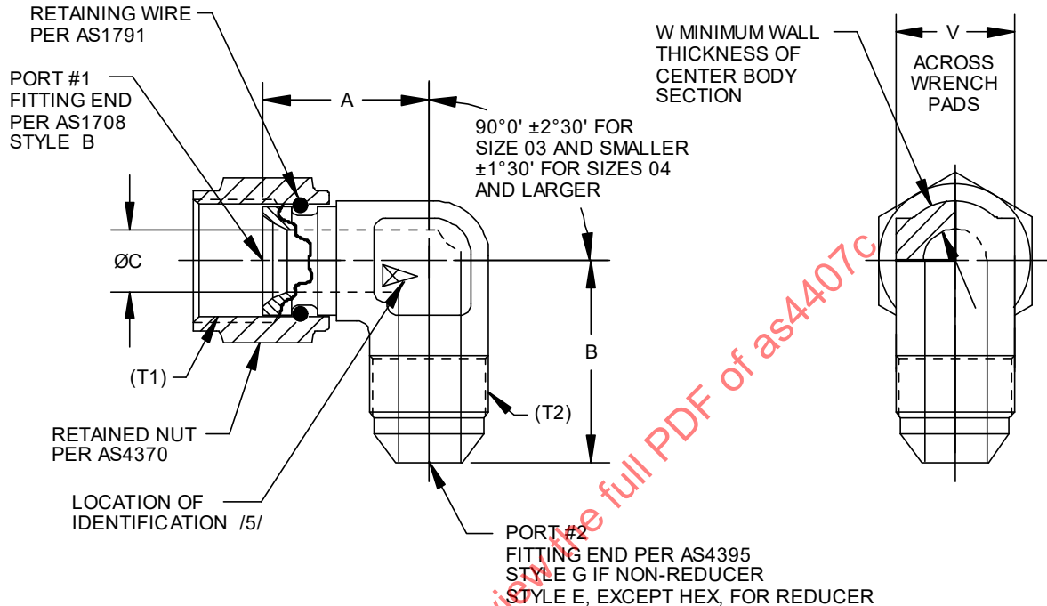
FIGURE 1 - FITTING ASSEMBLY, ELBOW 90°
