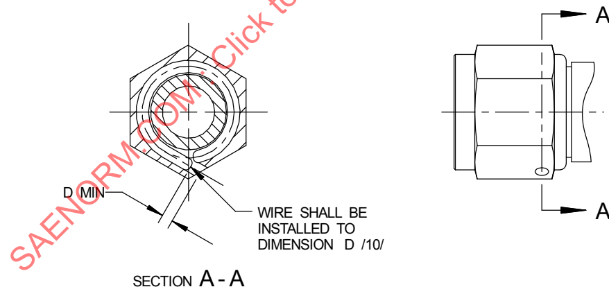
FIGURE 2 - INSTALLATION, RETAINED NUT AND RETAINING WIRE
