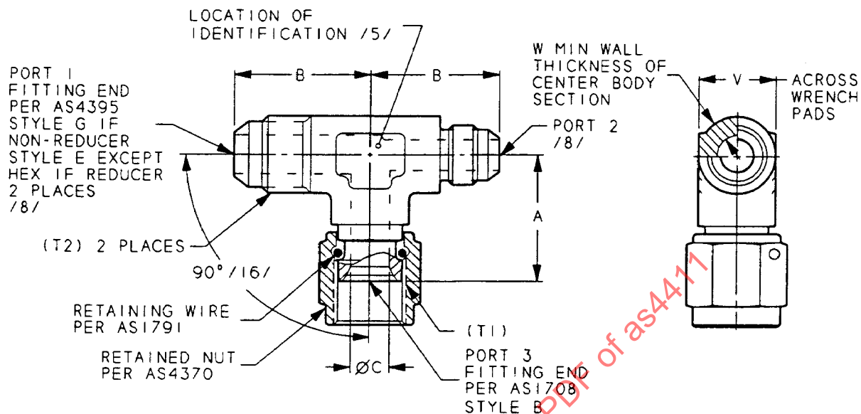
FIGURE 1 - FITTING ASSEMBLY, TEE
