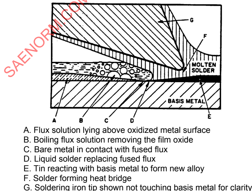
FIGURE 4 - SOLDER APPLICATION AND BRIDGING (SEE 4.9.5)
