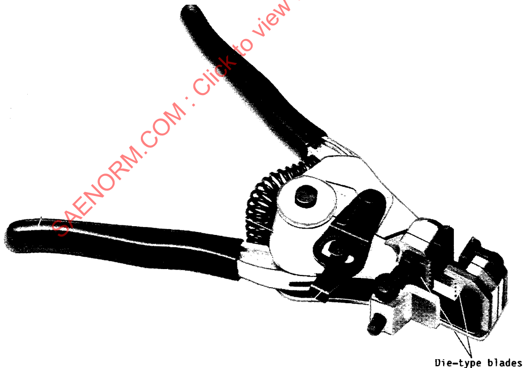
FIGURE 2 - AS5756 MECHANICAL HAND WIRE STRIPPER (SEE 4.6.2.2)
