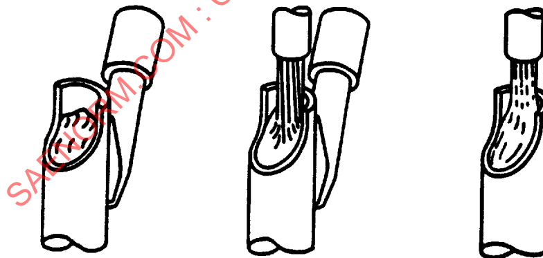
FIGURE 7 - SOLDERING OF HOLLOW CYLINDRICAL CONNECTIONS (SEE 4.9.5.1)
