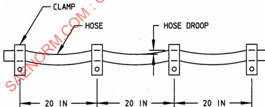
FIGURE 2 - Hose Droop
