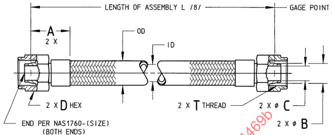
FIGURE 1 - HOSE ASSEMBLY
