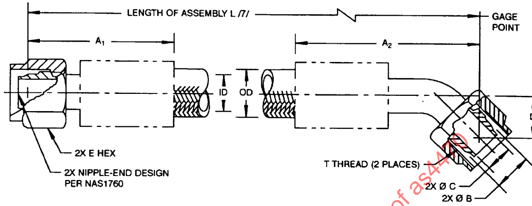
FIGURE 1 - HOSE ASSEMBLY
