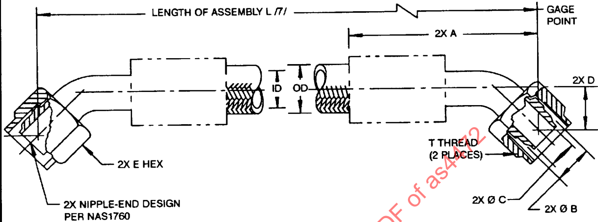
FIGURE 1 - HOSE ASSEMBLY
