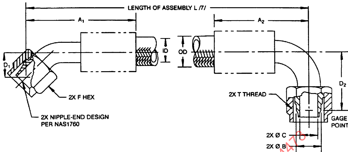
FIGURE 1 - HOSE ASSEMBLY
