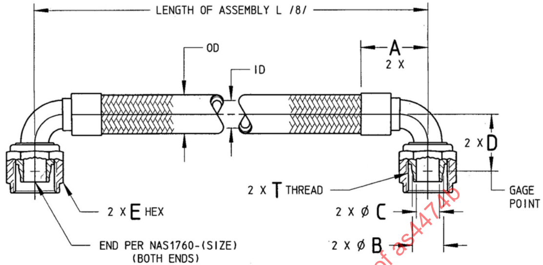
FIGURE 1 - HOSE ASSEMBLY
