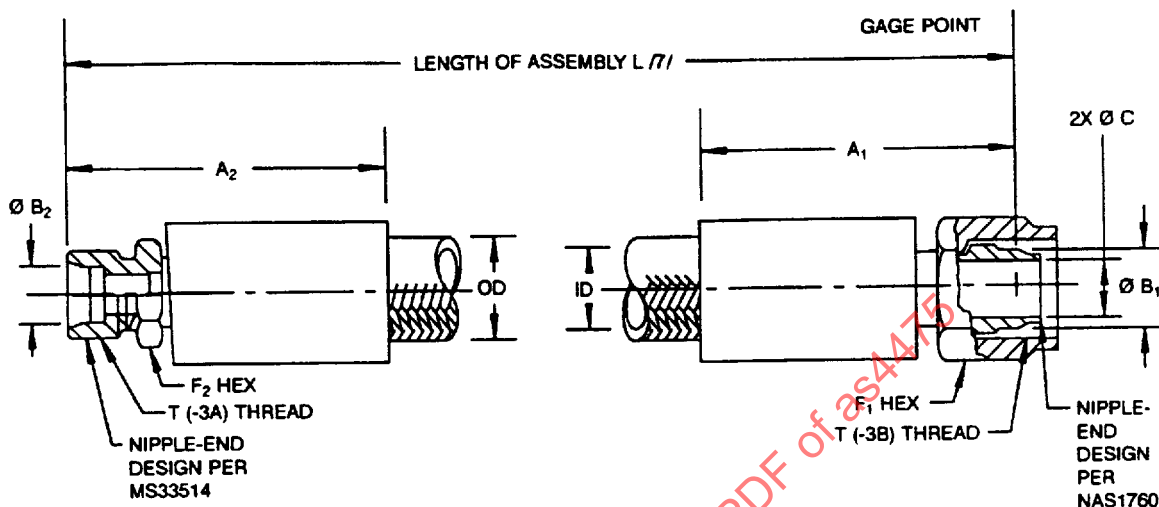
FIGURE 1 - HOSE ASSEMBLY
