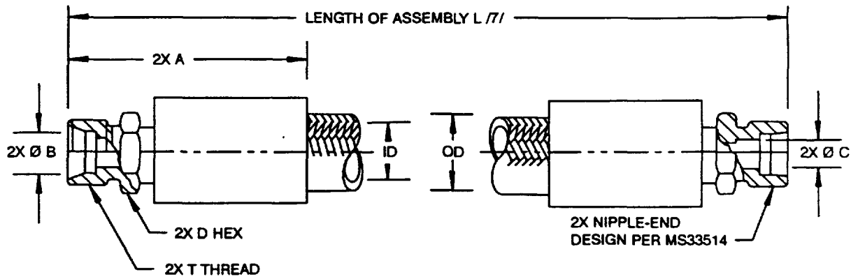
FIGURE 1 - HOSE ASSEMBLY
