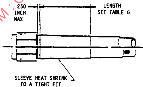
FIGURE 2 - SPIRAL ABRASION COVER /6/
