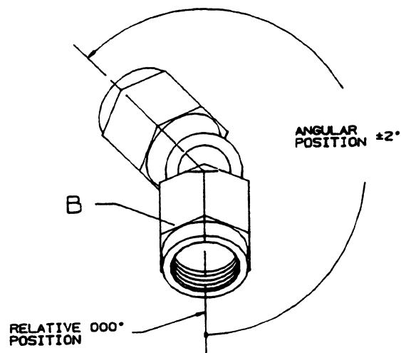
FIGURE 3 - FITTING ANGULAR ORIENTATION /16/
