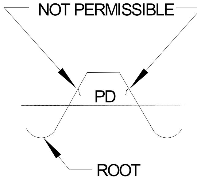
Figure 6 - Laps above pitch diameter extending towards root, rolled thread
