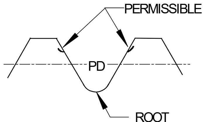
Figure 5 - Laps above pitch diameter extending towards crest, rolled thread
