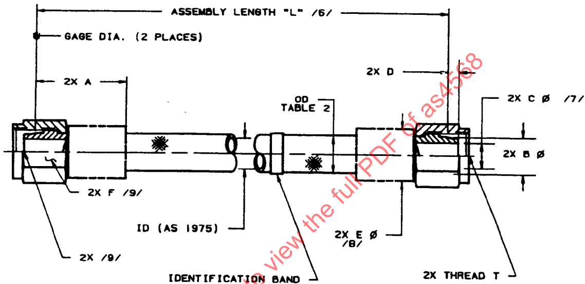
FIGURE 1 - HOSE ASSEMBLY, STRAIGHT TO STRAIGHT
