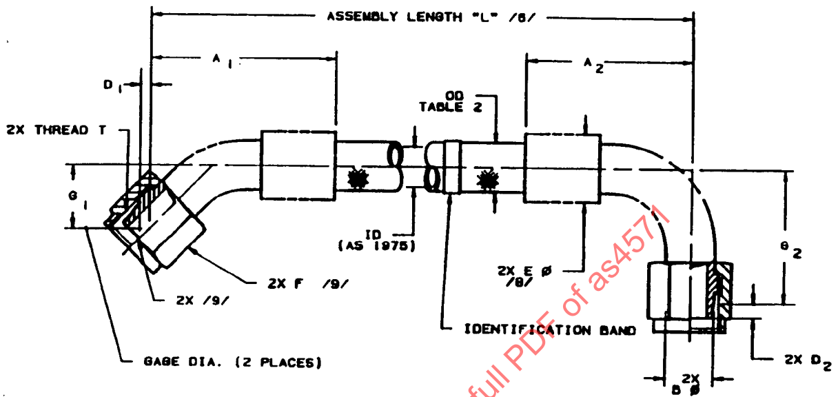
FIGURE 1 - HOSE ASSEMBLY, 45° ELBOW TO 90° ELBOW
