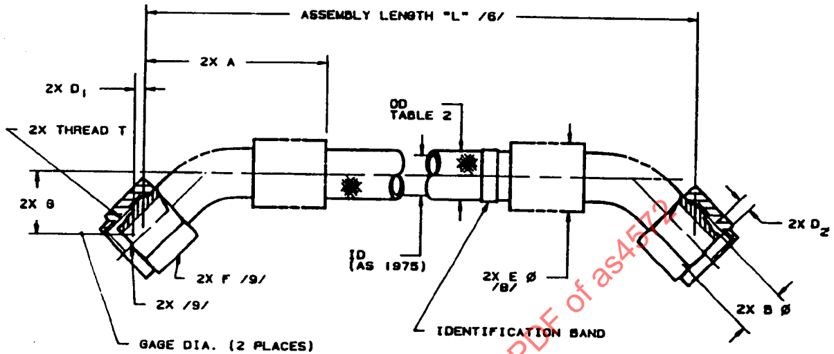
FIGURE 1 - HOSE ASSEMBLY, 45° ELBOW TO 45° ELBOW
