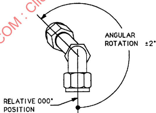
FIGURE 2 - ASSEMBLY ORIENTATION
