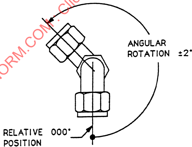
FIGURE 2 - ASSEMBLY ORIENTATION
