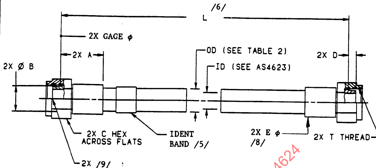
FIGURE 1 - HOSE ASSEMBLY, STRAIGHT TO STRAIGHT
