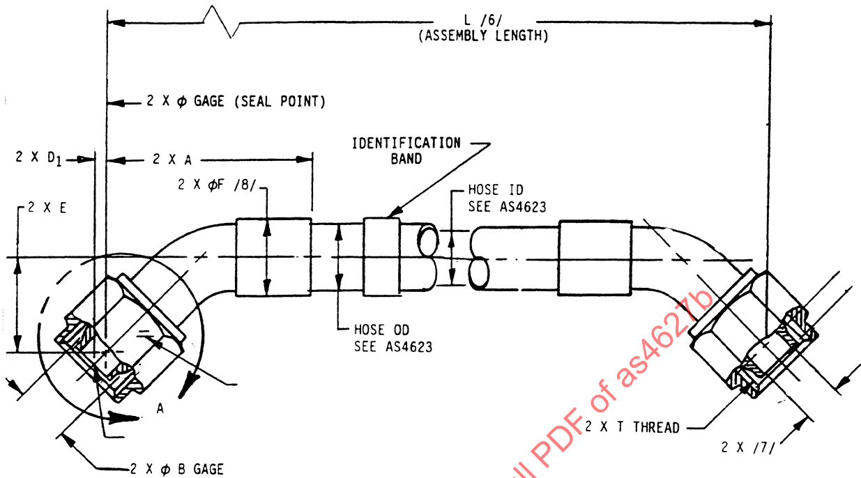
FIGURE 1 - HOSE ASSEMBLY, 45° ELBOW TO 45° ELBOW
