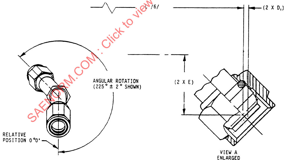
FIGURE 2 - FITTING ORIENTATION /19/
