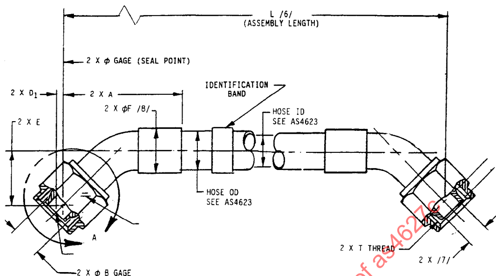
FIGURE 1 - HOSE ASSEMBLY, 45° ELBOW TO 45° ELBOW
