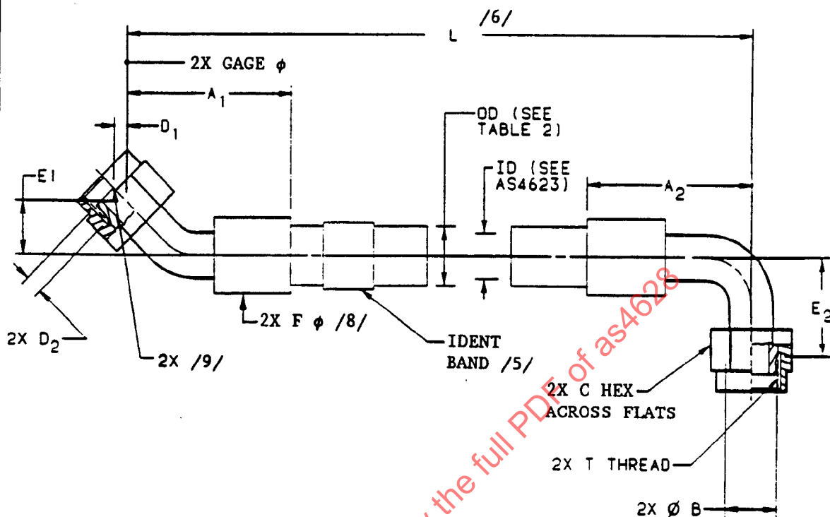
FIGURE 1 - HOSE ASSEMBLY, 45° ELBOW TO 90° ELBOW
