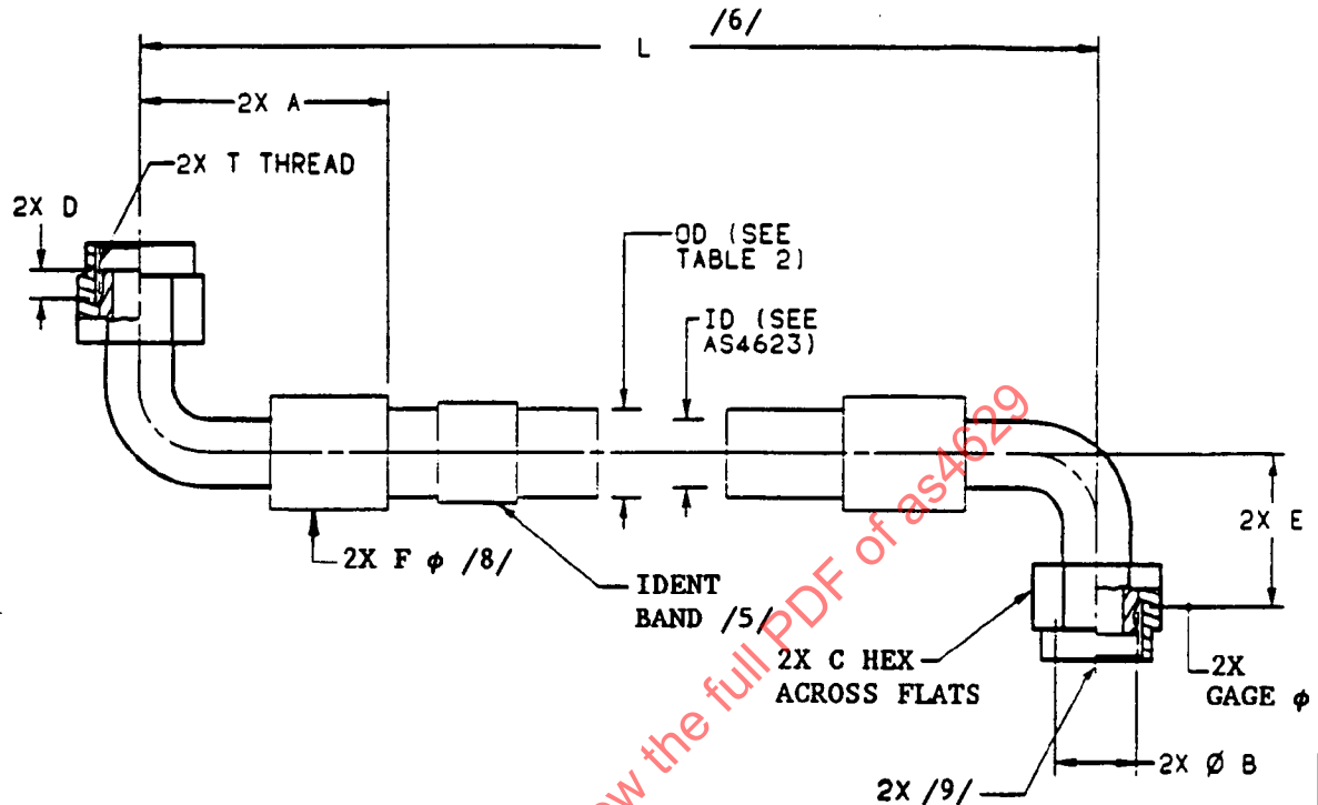
FIGURE 1 - HOSE ASSEMBLY, 90° ELBOW TO 90° ELBOW
