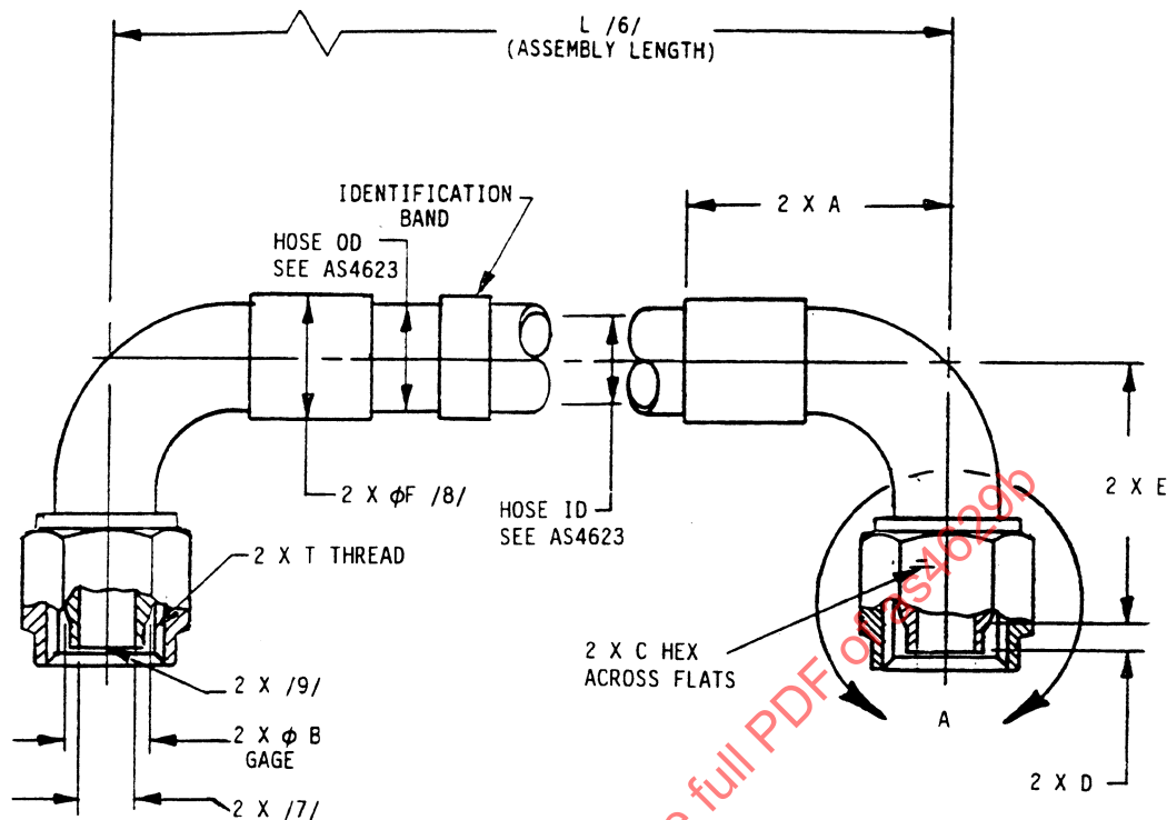
FIGURE 1 - HOSE ASSEMBLY, 90° ELBOW TO 90° ELBOW
