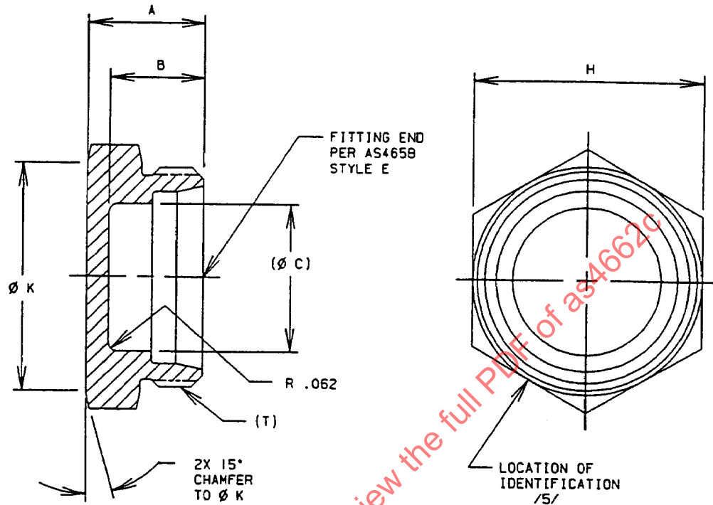
FIGURE 1 - FITTING, PLUG, SHORT FLARELESS
