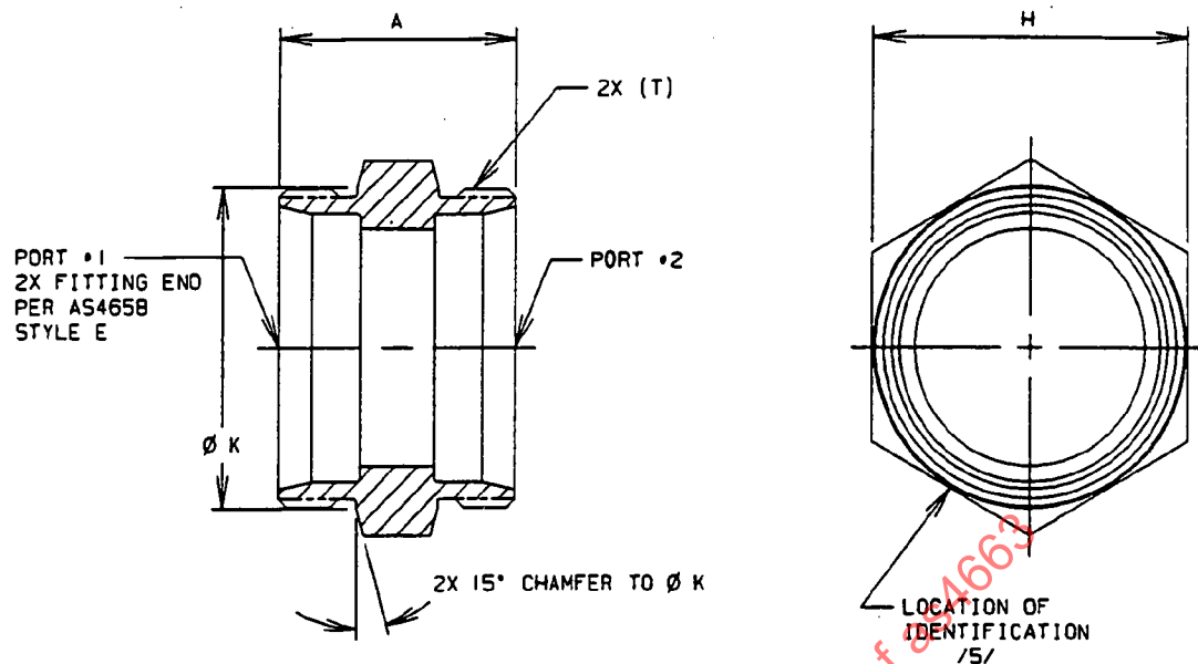
FIGURE 1 - UNION, SHORT FLARELESS
